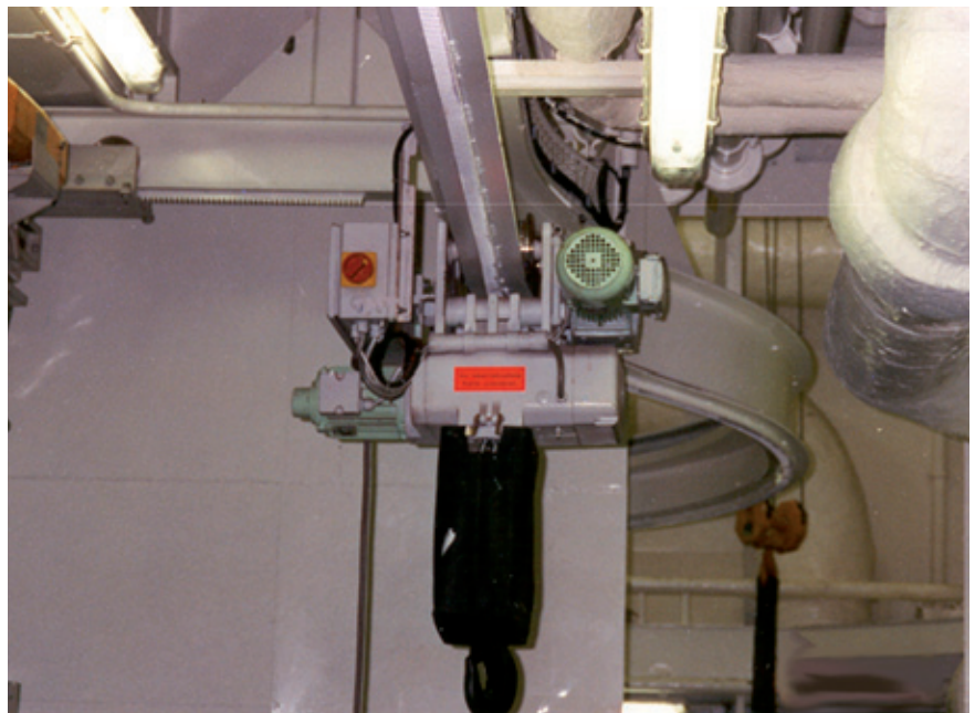
SWL 5t Radius 2250mm Class RINA
