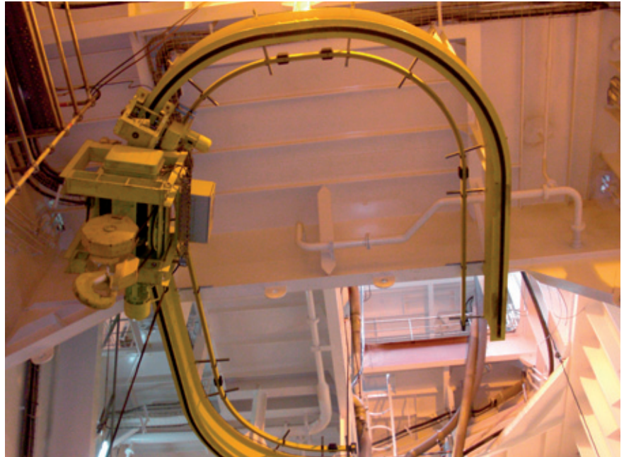
SWL 25t Radius 1800mm Class BV
